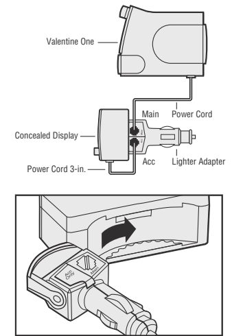
Lighter Adapter slides into place.
