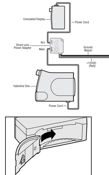
Mounting plate slides into place.
