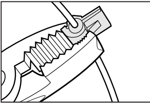
Pinch connector around power wire.
